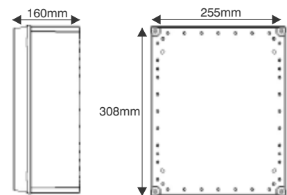
FIBC Power Supply / Interface Unit
